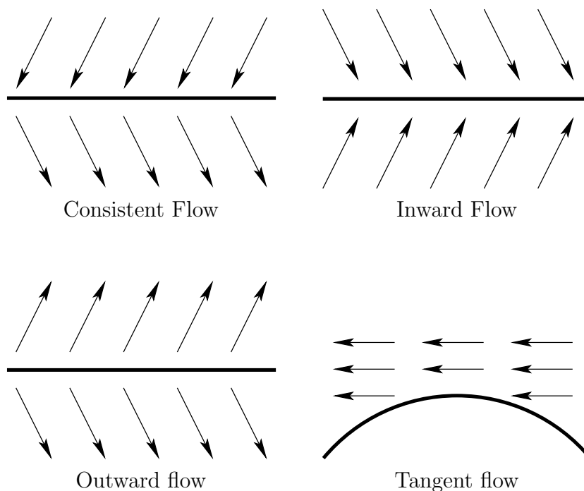
Figure 8.7: Different kinds of flows around a switching boundary.
